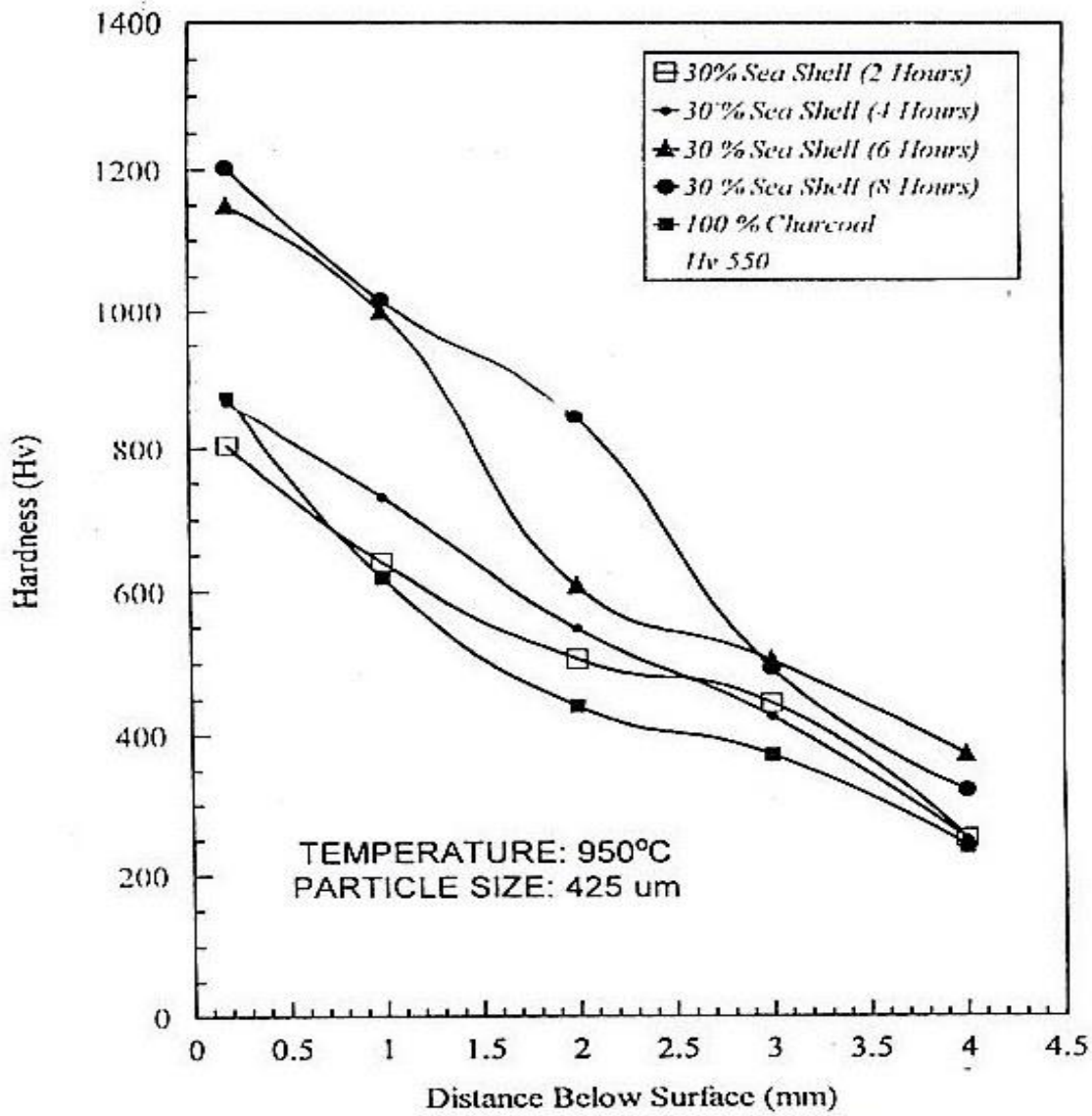
Figure 2: Effect of Holding Time on the Carburizing Kinetics Using 30 % Sea Shell at 950 °C
