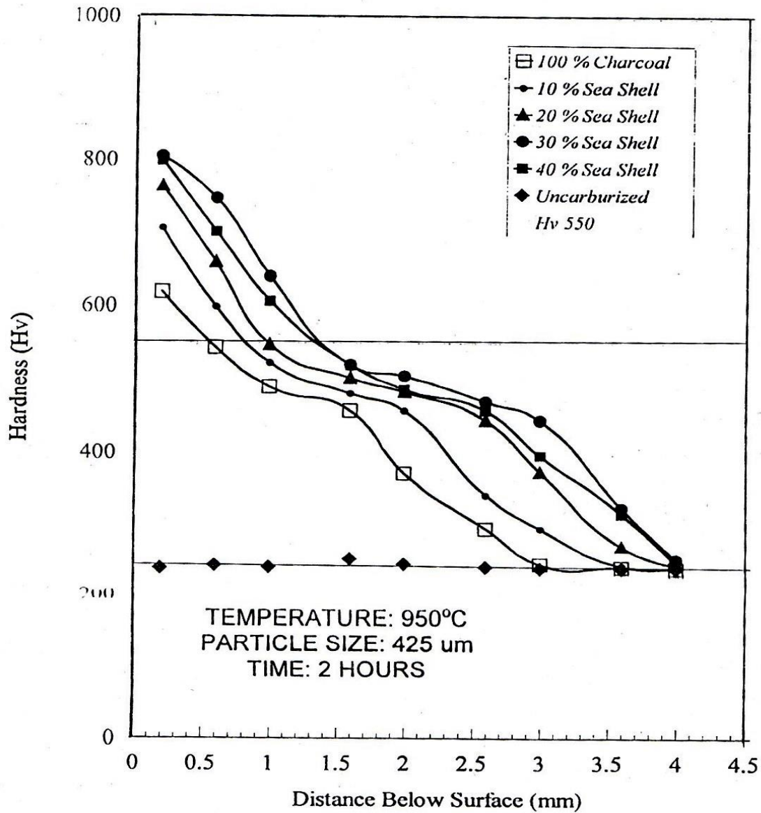
Figure 1: Graphical - Determination of Case Depth using Hardness Profiles and distance data for Different Carburizing Compounds after 2 Hours at 950 °C
